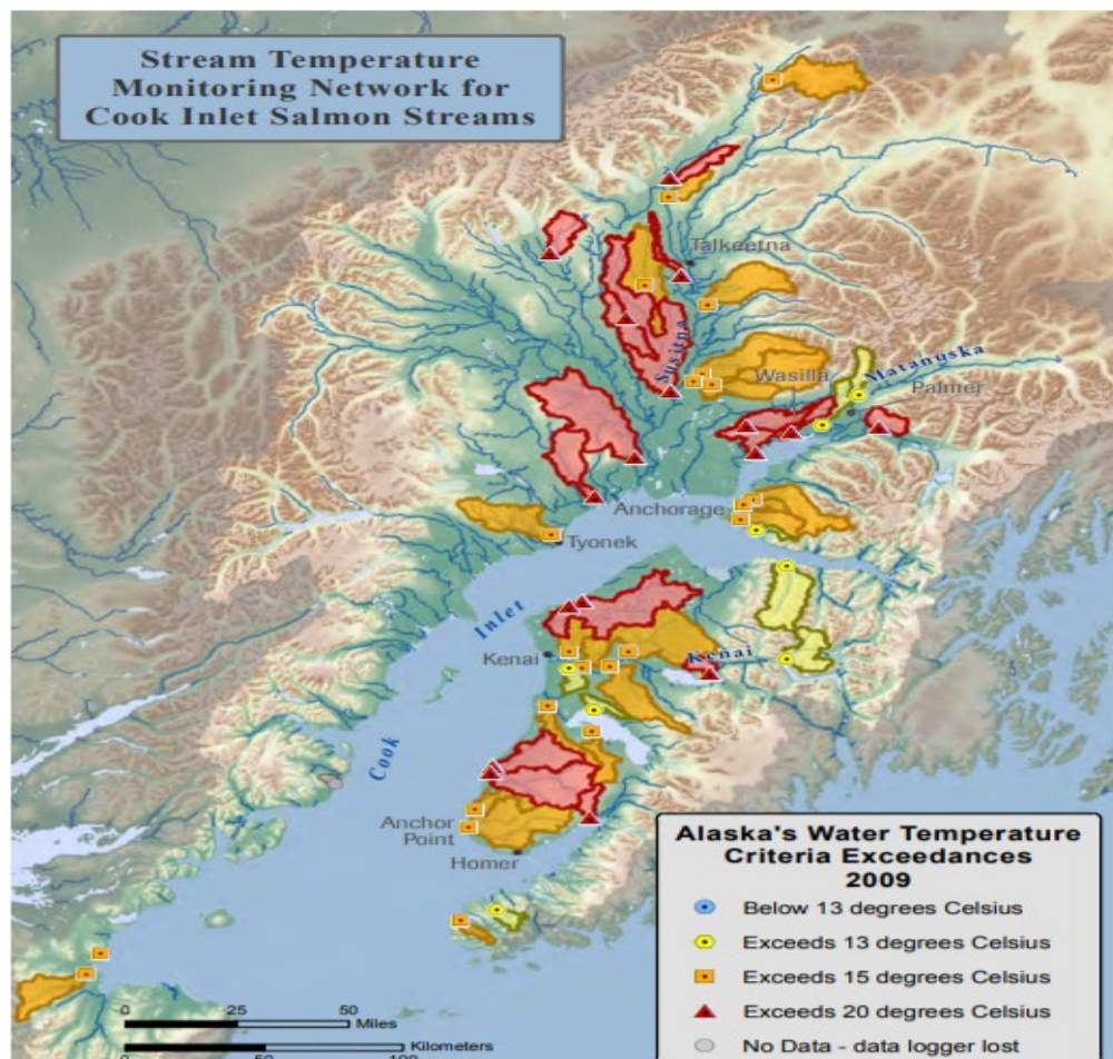
Figure 22: Stream temperatures monitored in the Cook Inlet basin, Alaska. Nearly all exceeded maximum tolerance levels for salmon at least part of the summer. Source: Sea Grant Alaska 2016
