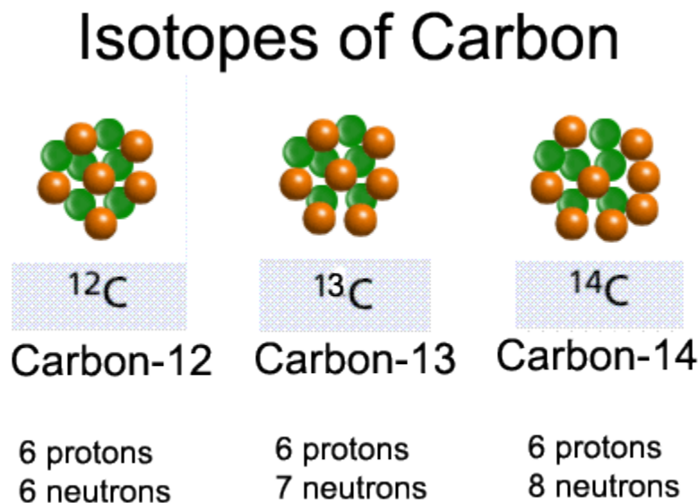
Figure 5: The Isotopes of Carbon and the configuration of protons and neutrons. (Source: Socratic.org)
