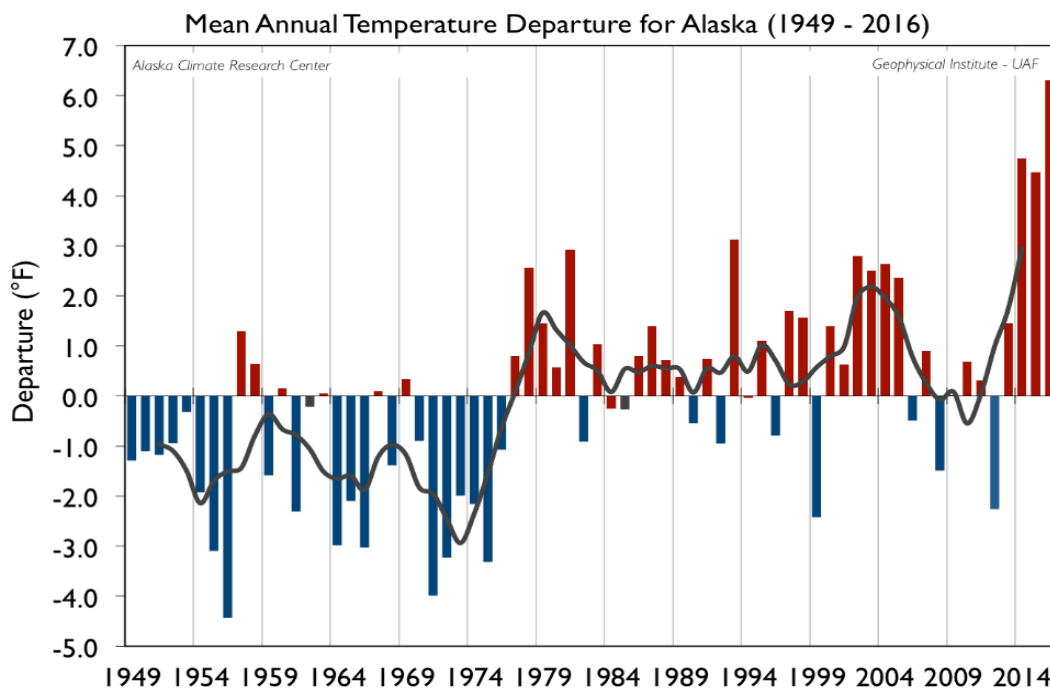
Figure 2: Mean Annual Temperature Departure for Alaska. The year is shown on the horizontal axis (x-axis) increasing from 1949 on the left to 2016 in the right. Temperature Departures for Alaska are shown on the left vertical axis (y-axis) and are represented by the blue and red bars on the graph. (Source: The Alaska Climate Research Center).
