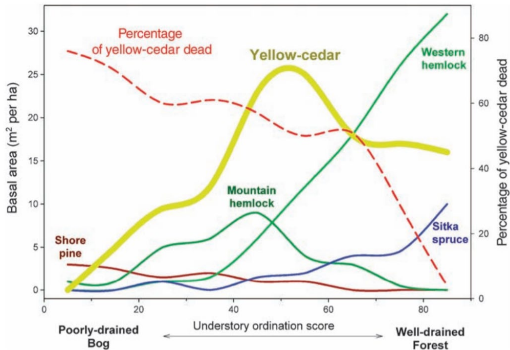
Figure 14. Yellow-cedar's optimum edaphic niche and the occurrence of yellow-cedar mortality along the soil-drainage gradient. The abundance (live basal area) of yellow-cedar and competing tree species was determined by splining the midpoint values from nine intervals along a range of soil-drainage levels indicated by understory plant composition expressed with ordination scores. (Source: BioScience)
